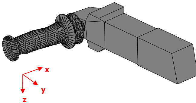
Figures: Schematic diagram showing the vibrating structure (left) vibration-attenuated auxiliary handle on an angle grinder (right)
